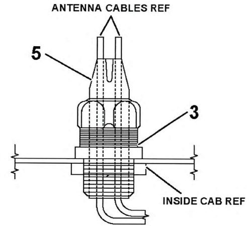
DETAIL C
